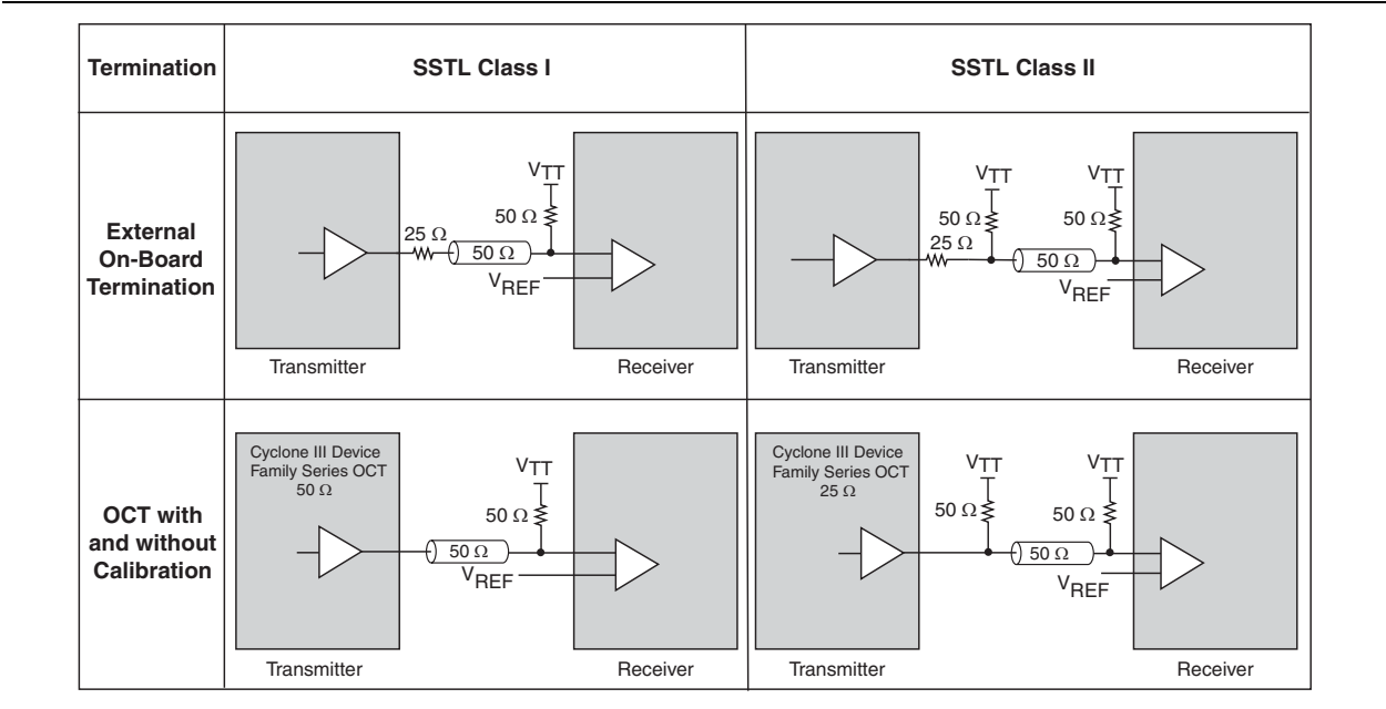
Figure 6-7. Cyclone III Device Family SSTL I/O Standard Termination
