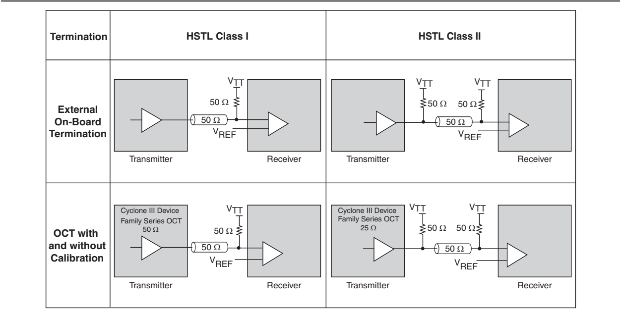
Figure 6-6. Cyclone III Device Family HSTL I/O Standard Termination
