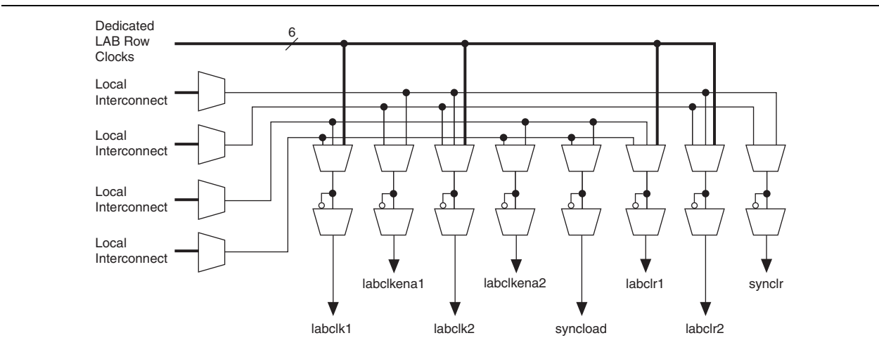
Figure 2-6. Cyclone III Device Family LAB-Wide Control Signals
